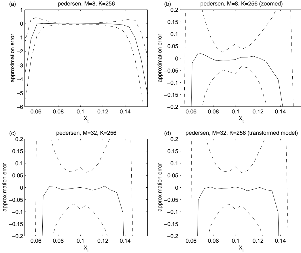
Figure 2: Approximation error, \log \hat{p}(X_t, t; X_s, s) - \log p(X_t, t; X_s, s) , using Pedersen's method given \Delta = t - s = 1/12 , X_s = 0.10 and \theta = (0.5, 0.06, 0.15) . The median and interquartile range over 1024 repetitions are plotted. The untransformed model is used in panels (a)-(c), and the transformed model is used in panel (d).
