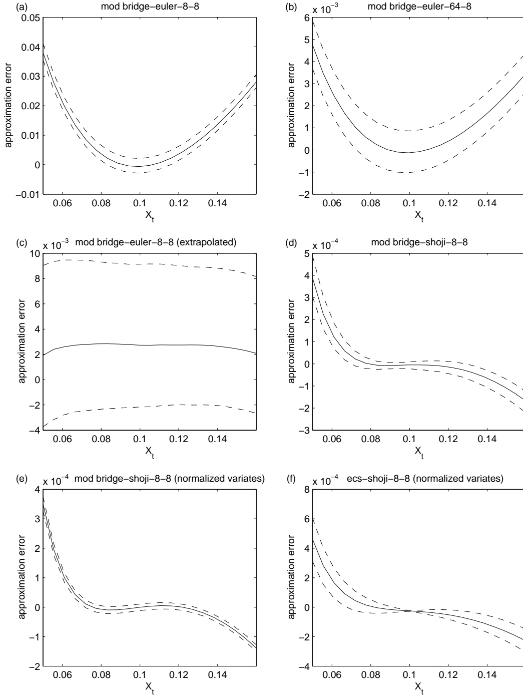
Figure 9: Approximation error, \log \hat{p}(X_t, t; X_s, s) - \log p(X_t, t; X_s, s) , for various simulated likelihood schemes given \Delta = t - s = 1/12 , X_s = 0.10 and \theta = (0.5, 0.06, 0.15) . The median and interquartile range over 128 repetitions are plotted. The transformed model is used.
