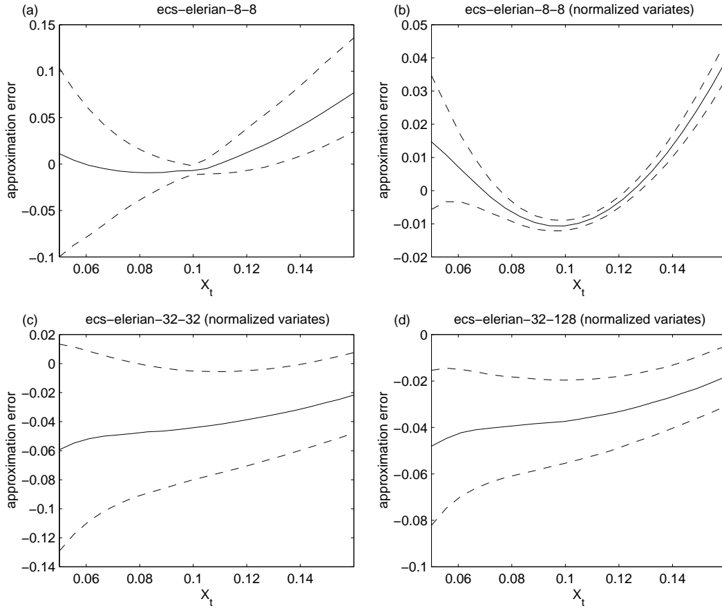
Figure 8: Approximation error, \log \hat{p}(X_t, t; X_s, s) - \log p(X_t, t; X_s, s) , for various simulated likelihood schemes given \Delta = t - s = 1/12 , X_s = 0.10 and \theta = (0.5, 0.06, 0.15) . The median and interquartile range over 128 repetitions are plotted. The untransformed model is used.
