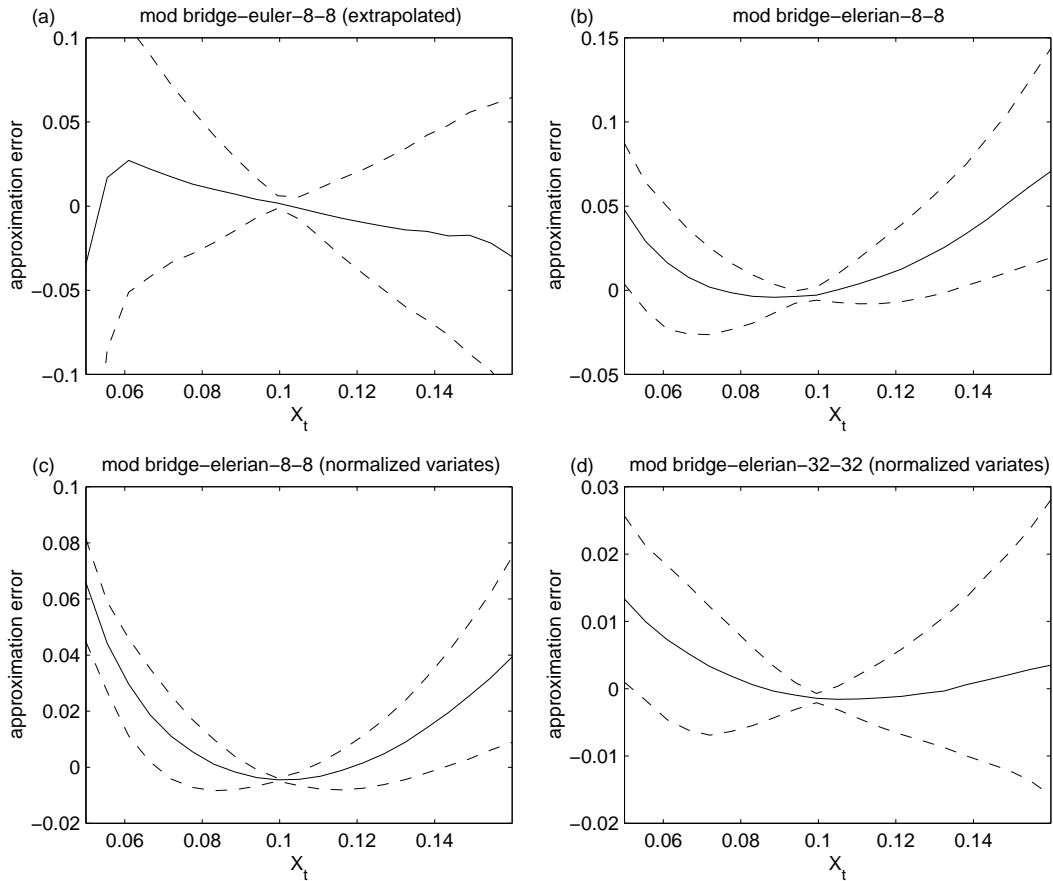
Figure 7: Approximation error, \log \hat{p}(X_t, t; X_s, s) - \log p(X_t, t; X_s, s) , for various simulated likelihood schemes given \Delta = t - s = 1/12 , X_s = 0.10 and \theta = (0.5, 0.06, 0.15) . The median and interquartile range over 128 repetitions are plotted. The untransformed model is used.
