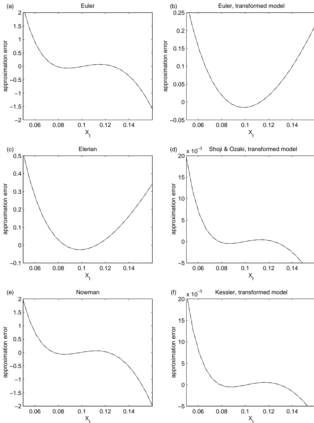
Figure 5: Approximation error, \log \hat{p}(X_t, t; X_s, s) - \log p(X_t, t; X_s, s) , for various schemes without using simulation (i.e., M = 1 , K = 1 ) given \Delta = t - s = 1/12 , X_s = 0.10 and \theta = (0.5, 0.06, 0.15) .
