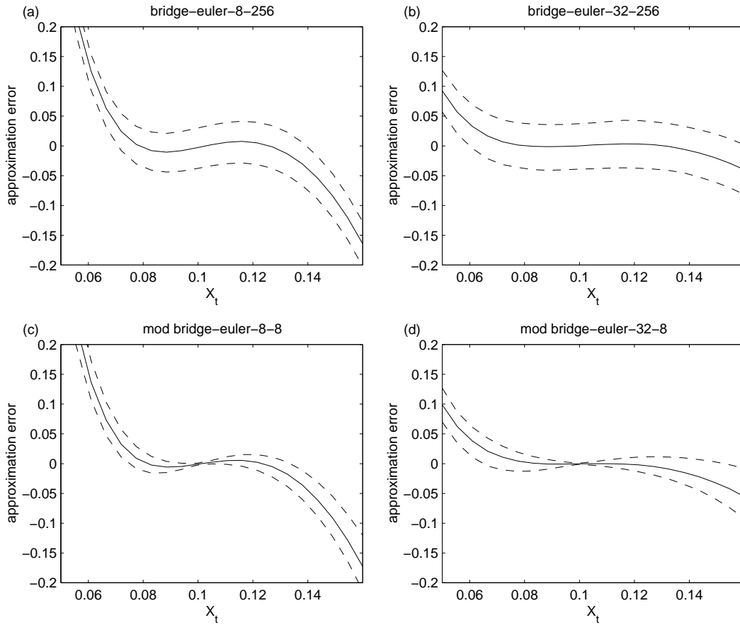
Figure 6: Approximation error, \log \hat{p}(X_t, t; X_s, s) - \log p(X_t, t; X_s, s) , for various simulated likelihood schemes given \Delta = t - s = 1/12 , X_s = 0.10 and \theta = (0.5, 0.06, 0.15) . The median and interquartile range over 128 repetitions are plotted. The untransformed model is used.
