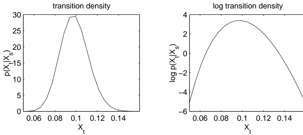
Figure 1: True transition density and log transition density for the CIR model given \Delta = t - s = 1/12 , X_s = 0.10 and \theta = (0.5, 0.06, 0.15) .
